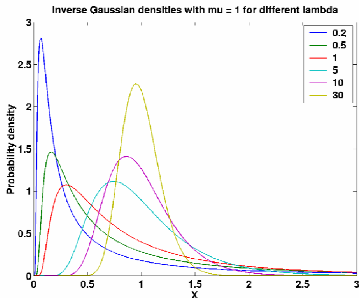
Figure 3K. Examples of inverse Gaussian probability densities.
